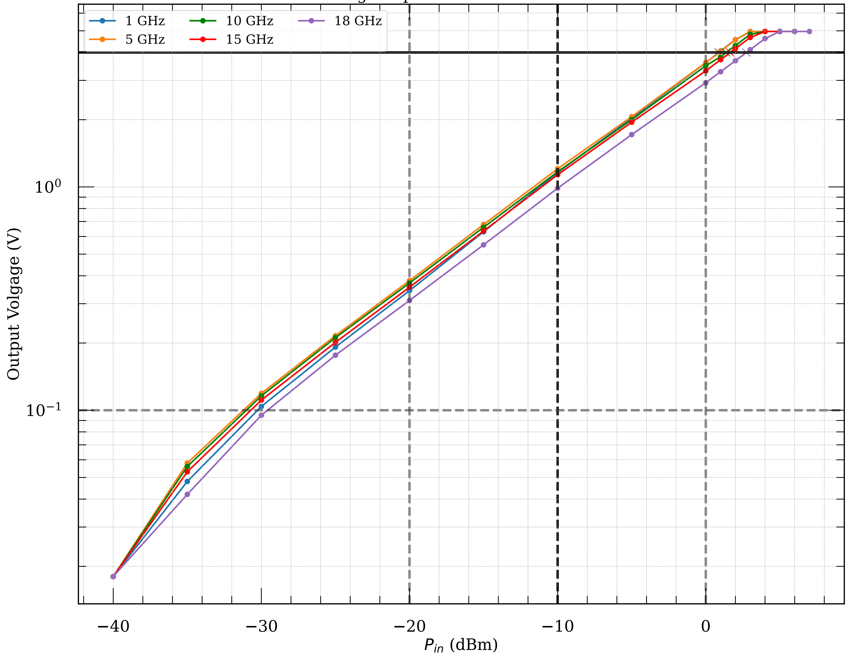
Measured voltage-to-power curve of detector module074
